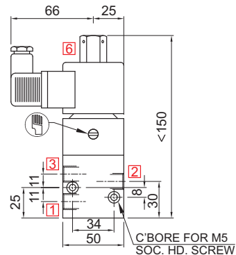
PLUG IN SOLENOID TYPE 25
