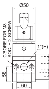
PLUG IN SOLENOID TYPE 22/ 25
