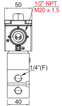
TERMINAL BOX/ Ex d/ LARGE ENCLOSURE, TYPE 16, 19, 37, 39
