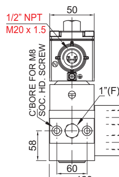
TERMINAL BOX/ Ex d LARGE ENCLOSURE, TYPE 16, 19, 37, 39
