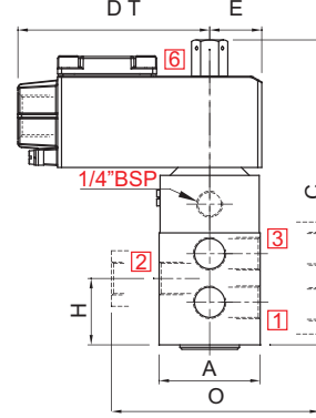
TERMINAL BOX/ Ex d LARGE ENCLOSURE, TYPE 16, 19, 37, 39
