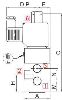
PLUG IN SOLENOID TYPE 22
