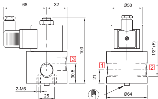
PLUG IN SOLENOID TYPE 25/ 22
