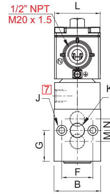
TERMINAL BOX/ Ex d LARGE ENCLOSURE, TYPE 16, 19, 37, 39
