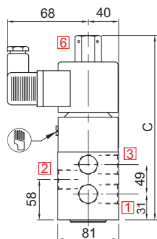
PLUG IN SOLENOID TYPE 22/ 25
