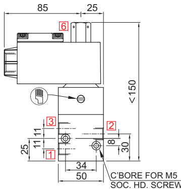
TERMINAL BOX/ Ex d/ TYPE 16, 19, 37, 39
