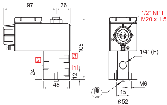
TERMINAL BOX/ Ex d/ LARGE ENCLOSURE, TYPE 16, 19, 37, 39, LC
