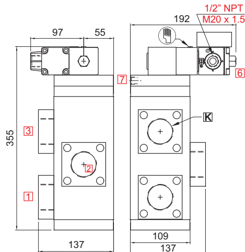
TERMINAL BOX/ Ex d. LARGE ENCLOSURE TYPE 16, 19, 37, 39, LC
