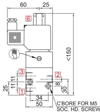
PLUG IN SOLENOID TYPE 22
