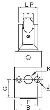
TERMINAL BOX/ Ex d/ TYPE 16, 19, 37, 39
