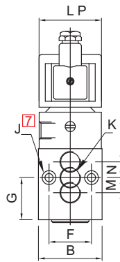
PLUG IN SOLENOID TYPE 22/ 25
