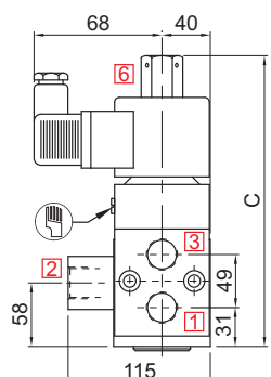
PLUG IN SOLENOID TYPE 22/ 25
