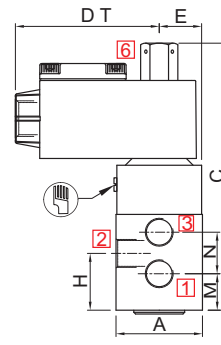
TERMINAL BOX/ Ex d. ENCLOSURE, TYPE 16, 19, 37, 39
