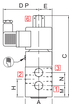
PLUG IN SOLENOID TYPE 25
