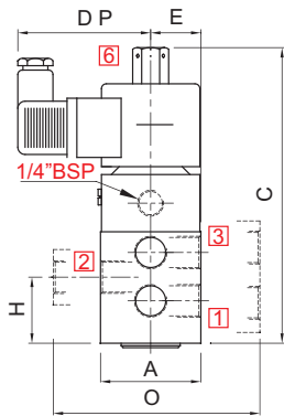
PLUG IN SOLENOID TYPE 25
