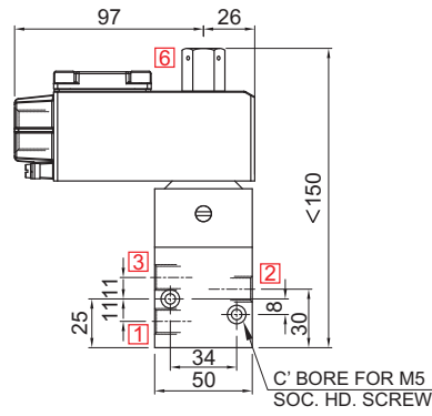
TERMINAL BOX/ Ex d/ LARGE ENCLOSURE, TYPE 16, 19, 37, 39
