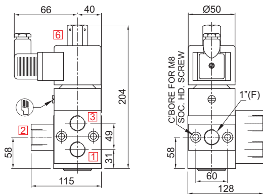
PLUG IN SOLENOID TYPE 22/ 25
