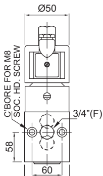
PLUG IN SOLENOID TYPE 22/ 25
