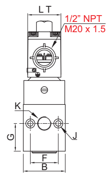
TERMINAL BOX/ Ex d. ENCLOSURE, TYPE 16, 19, 37, 39
